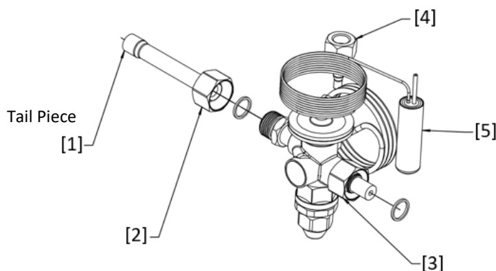
Figure 4 - TXV Installation
