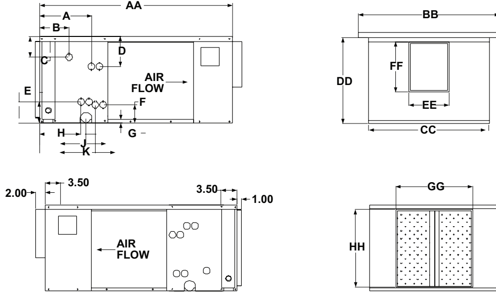
SHWX – UNIT DIMENSIONS
