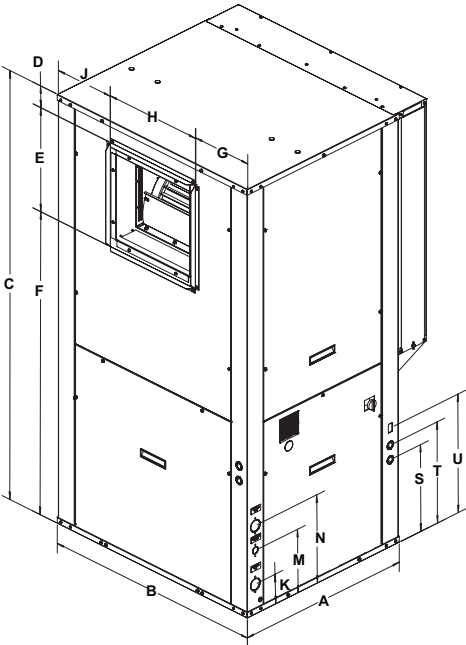
Straight Discharge Right Hand Unit
