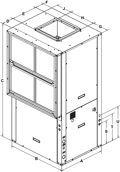
Top Discharge Right Hand Unit
