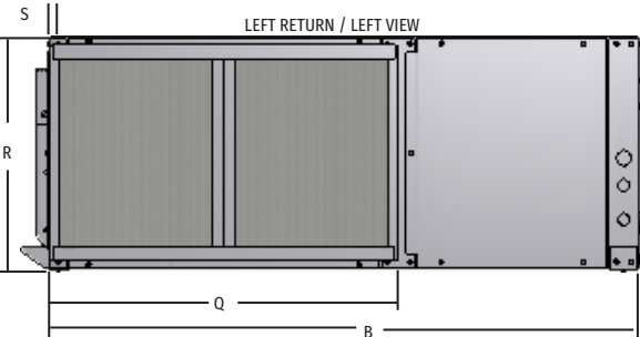
LEFT RETURN / STRAIGHT DISCHARGE
