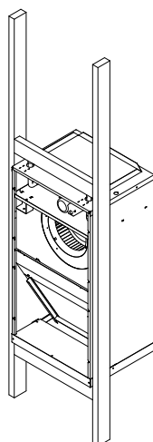
Typical Recessed Wall Installation
