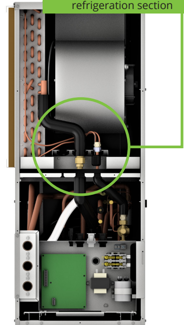
Disconnect couplings for refrigeration section
