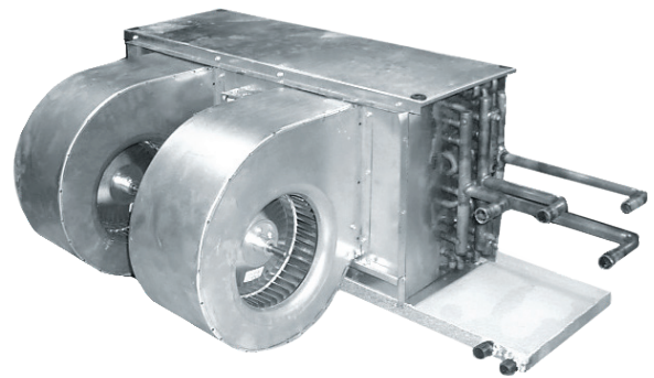
HYB Series Hydronic
