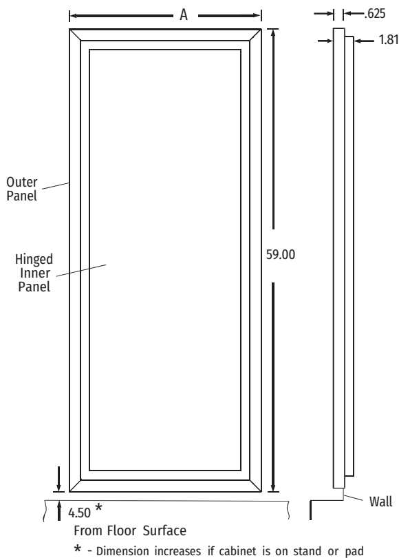
Front View Standard Panel
