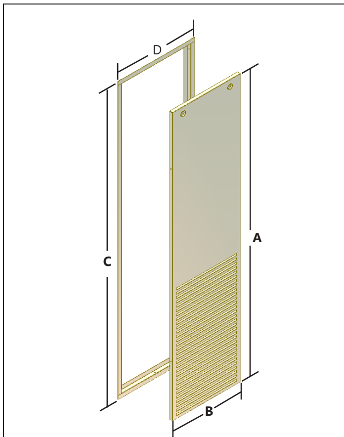
FLUSH MOUNT DIMENSIONS
