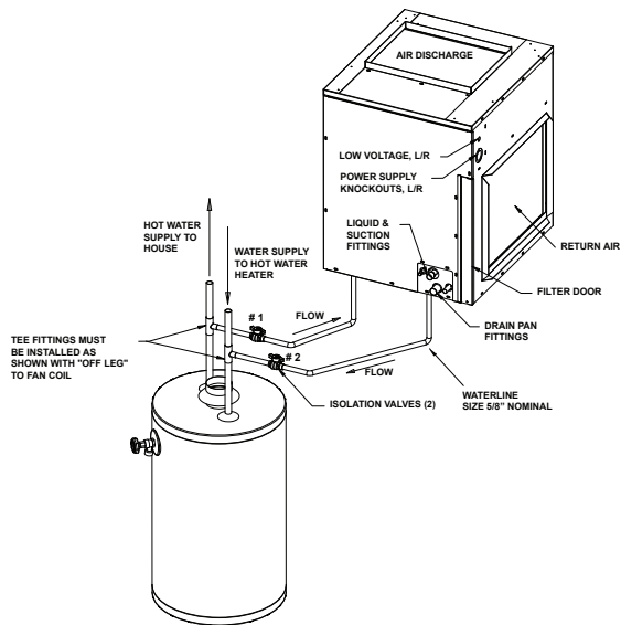
Typical connection to Tank-Type Water Heater
