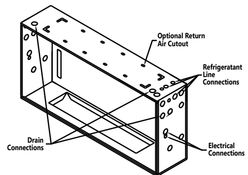
Connection Locations
